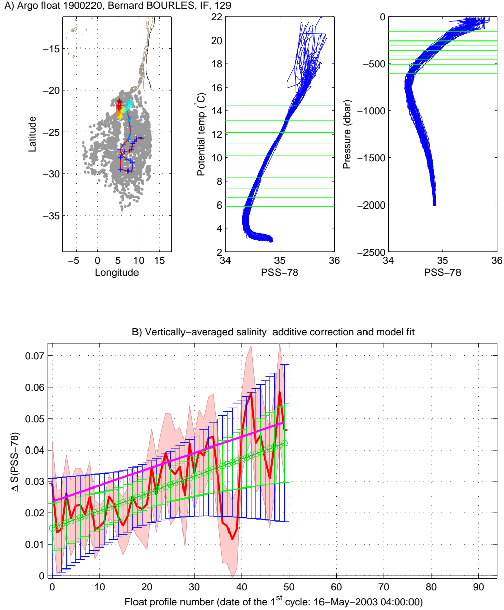
Figure 10: Float 1900220. Results of the OW method (configuration 129). Upper panels: Reference profiles used for the mapping (grey dots) are shown on a map along with the float trajectory. On the two most right-handed figures are displayed in green the ten most stable \theta levels used to compute the fit. Lower panel: vertically-averaged mapped salinities minus float salinities on the 10 most stable \theta levels (red line) and the offset obtained by a linear fit (green circles). The mapping errors are shaded in red. Green error bars show the fit error and blue error bars show the doubled fit error. The salinity correction currently available on the GDAC is displayed in magenta.
