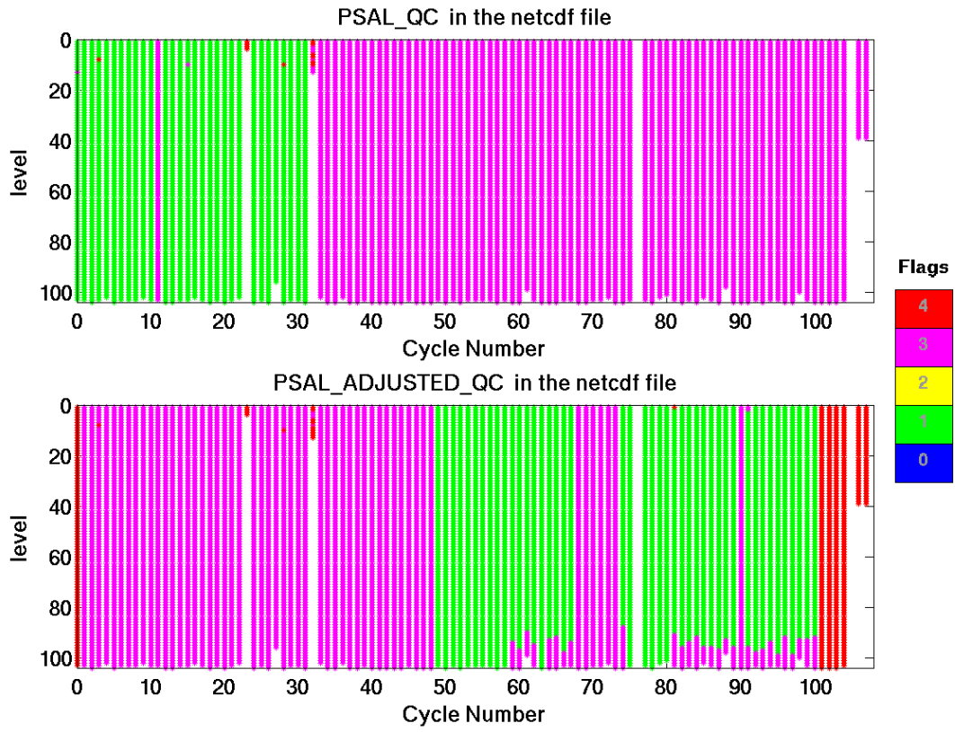
Figure 1: Float 1900205. Flags assigned to PSAL_QC and PSAL_ADJUSTED_QC in the netcdf file available on GDAC
