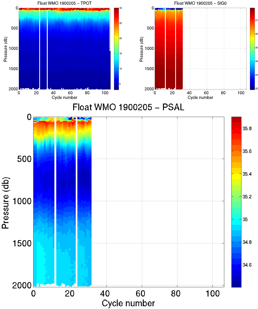
Figure 2: Float 1900205. Potential temperature, Sig0 and salinity sections along the float trajectory (raw data, bad data with quality flags > 2 are not plotted)
