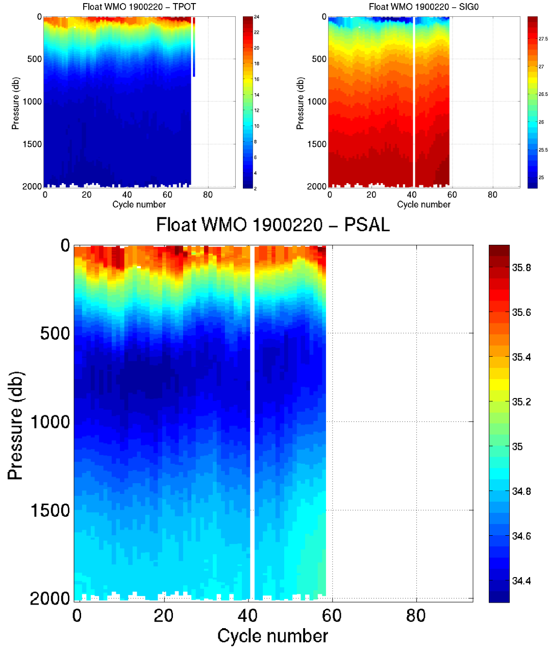
Figure 7: Float 1900220. Potential temperature, Sig0 and salinity sections along the float trajectory (raw data, bad data with quality flags > 2 are not plotted)
