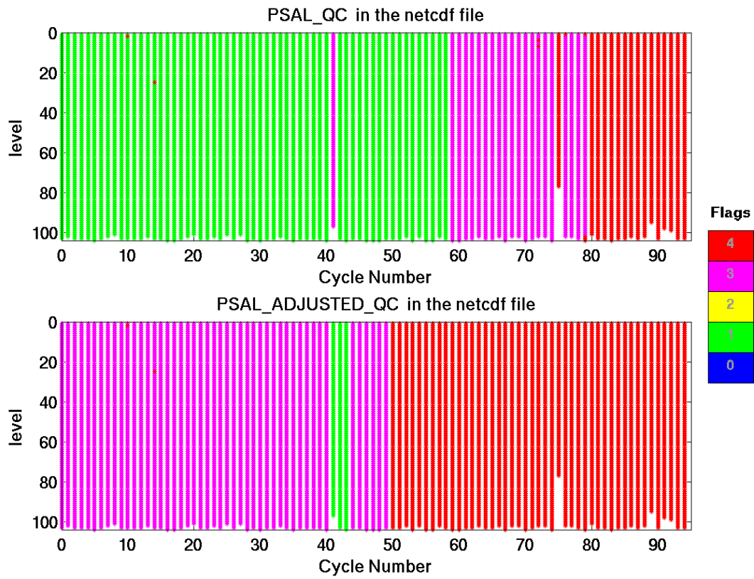
Figure 6: Float 1900220. Flags assigned to PSAL_QC and PSAL_ADJUSTED_QC in the netcdf file available on GDAC
