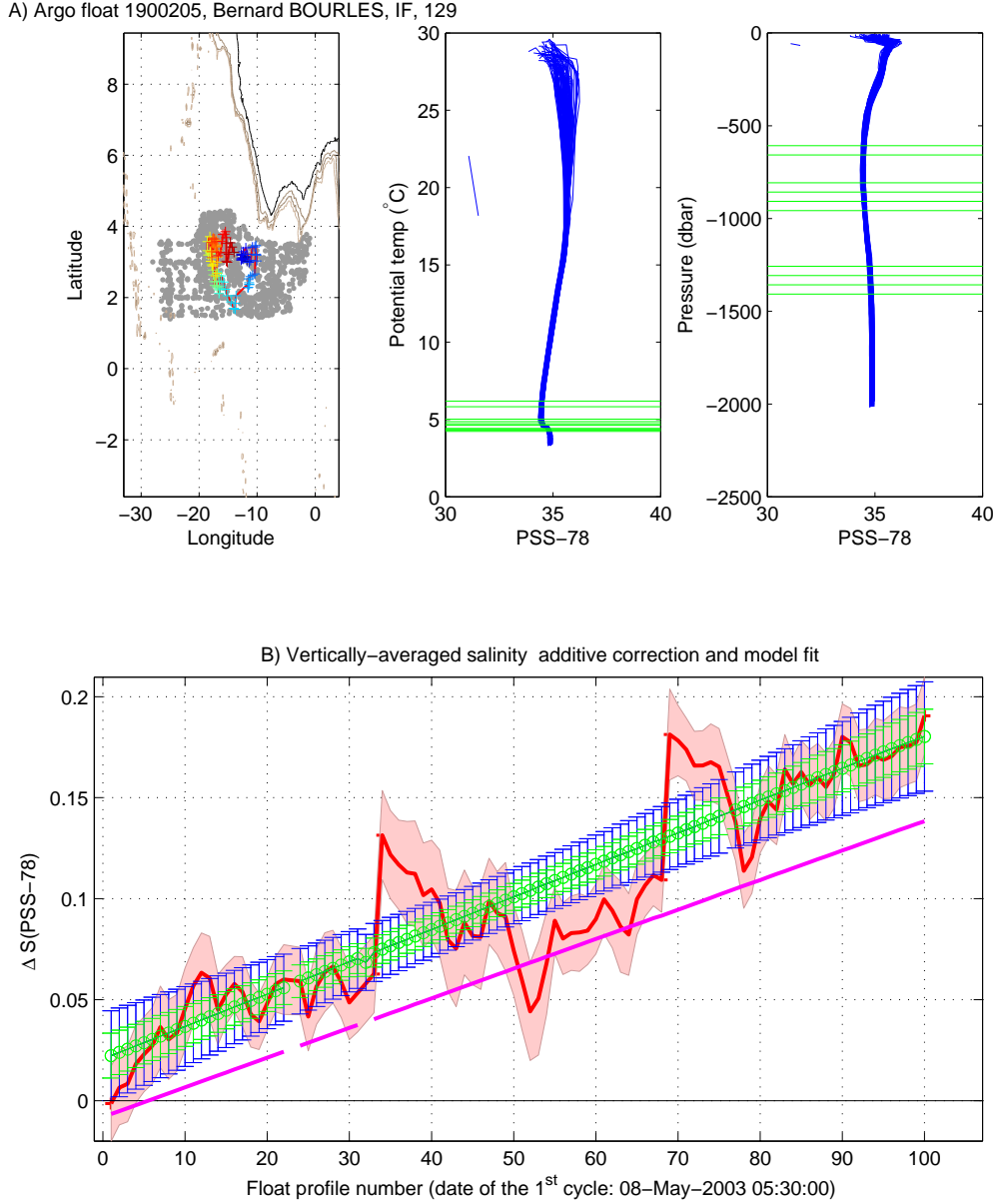
Figure 5: Float 1900205. Results of the OW method (configuration 129). Upper panels: Reference profiles used for the mapping (grey dots) are shown on a map along with the float trajectory. On the two most right-handed figures are displayed in green the ten most stable \theta levels used to compute the fit. Lower panel: vertically-averaged mapped salinities minus float salinities on the 10 most stable \theta levels (red line) and the offset obtained by a linear fit (green circles). The mapping errors are shaded in red. Green error bars show the fit error and blue error bars show the doubled fit error. The salinity correction currently available on the GDAC is displayed in magenta.
