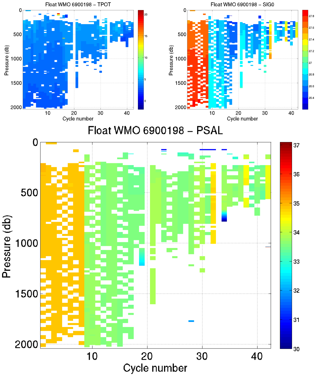
Figure 2: Float 6900198. Potential temperature, Sig0 and salinity sections along the float trajectory (raw data, bad data with quality flags > 2 are not plotted)
